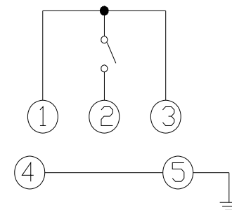
CIRCUIT DIAGRAM
